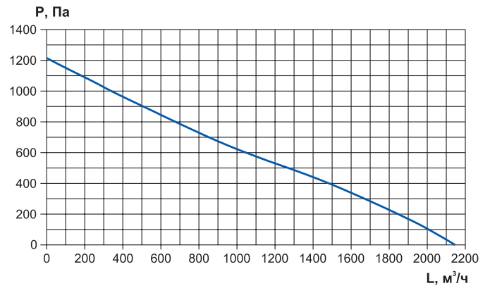
RWN-F-1000-EC
