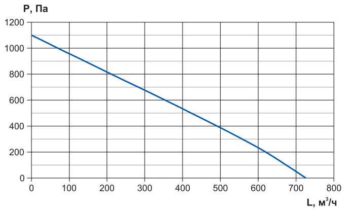
RWN-RR-1600-EC-Compact
