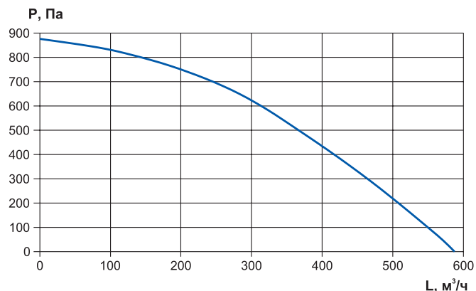
RWN-RR-600-EC-Classic
