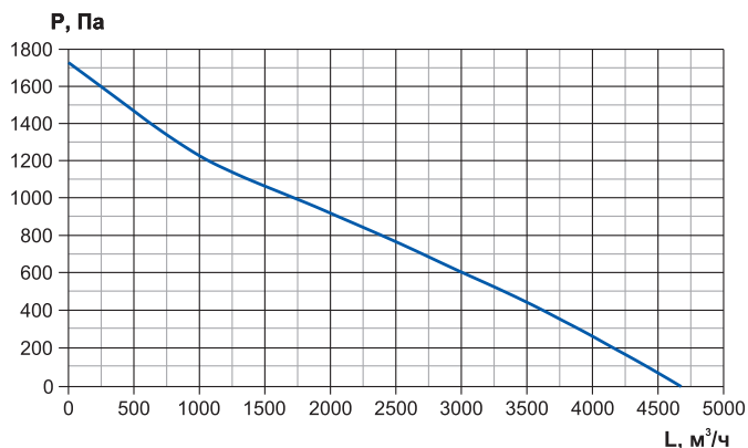
RWN-RP-6000-EC-Classic
