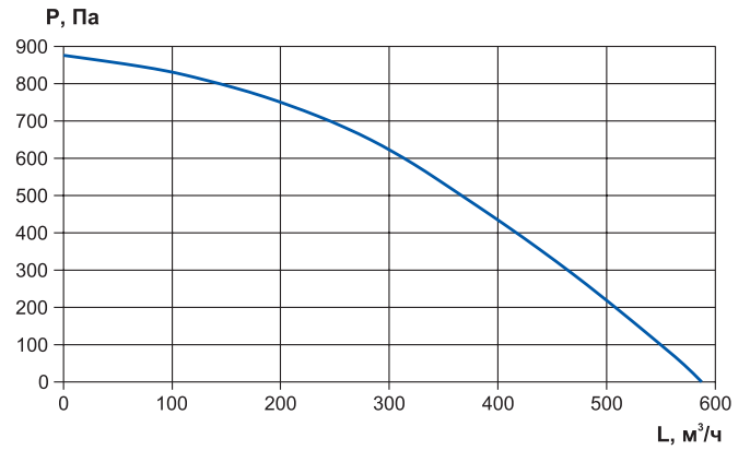
RWN-RR-600-EC-Compact
