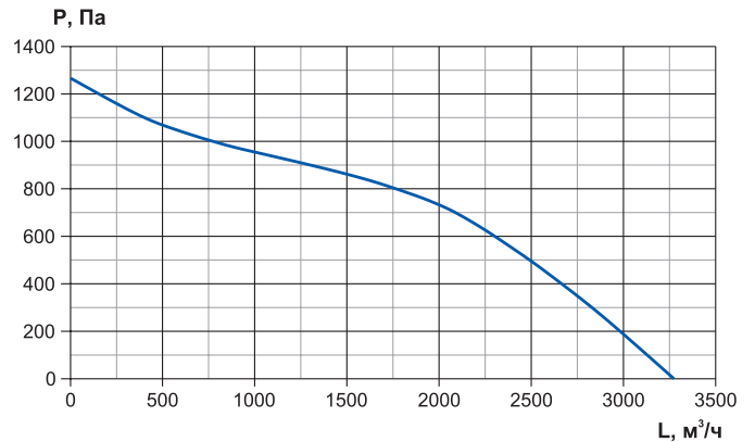
RWN-RR-4000-EC-Vertical
