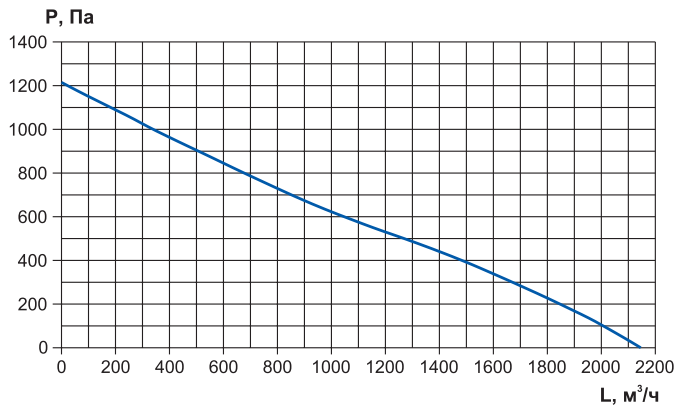
RWN-F-1500-EC
