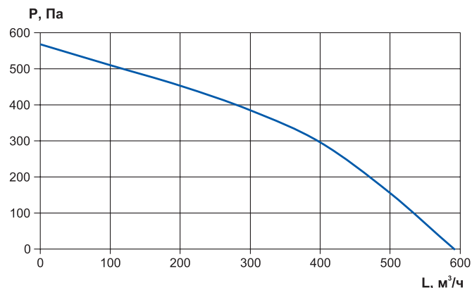
CV-SH-200-EC
